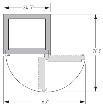
Door Swing Projections
